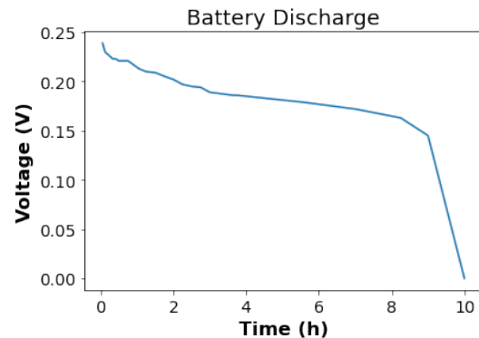
Figure 3: Battery Discharge
